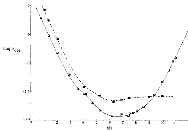
Figure 1. Log k_{\text{obs}} vs. pH rate profile for solvolysis of 4a-InH (—) and 4a-InMe (---): Solvent H 2 O (aerobic), 30°, \mu = 0.2 . Rate constants in min -1 . The E-2 elimination for 4a-InH may be seen in the slope of +1.
